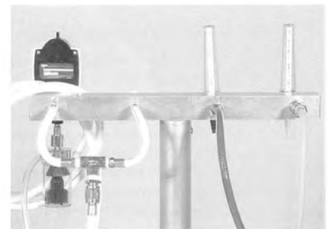
Rear of manifold for anesthesia/scavenger.
